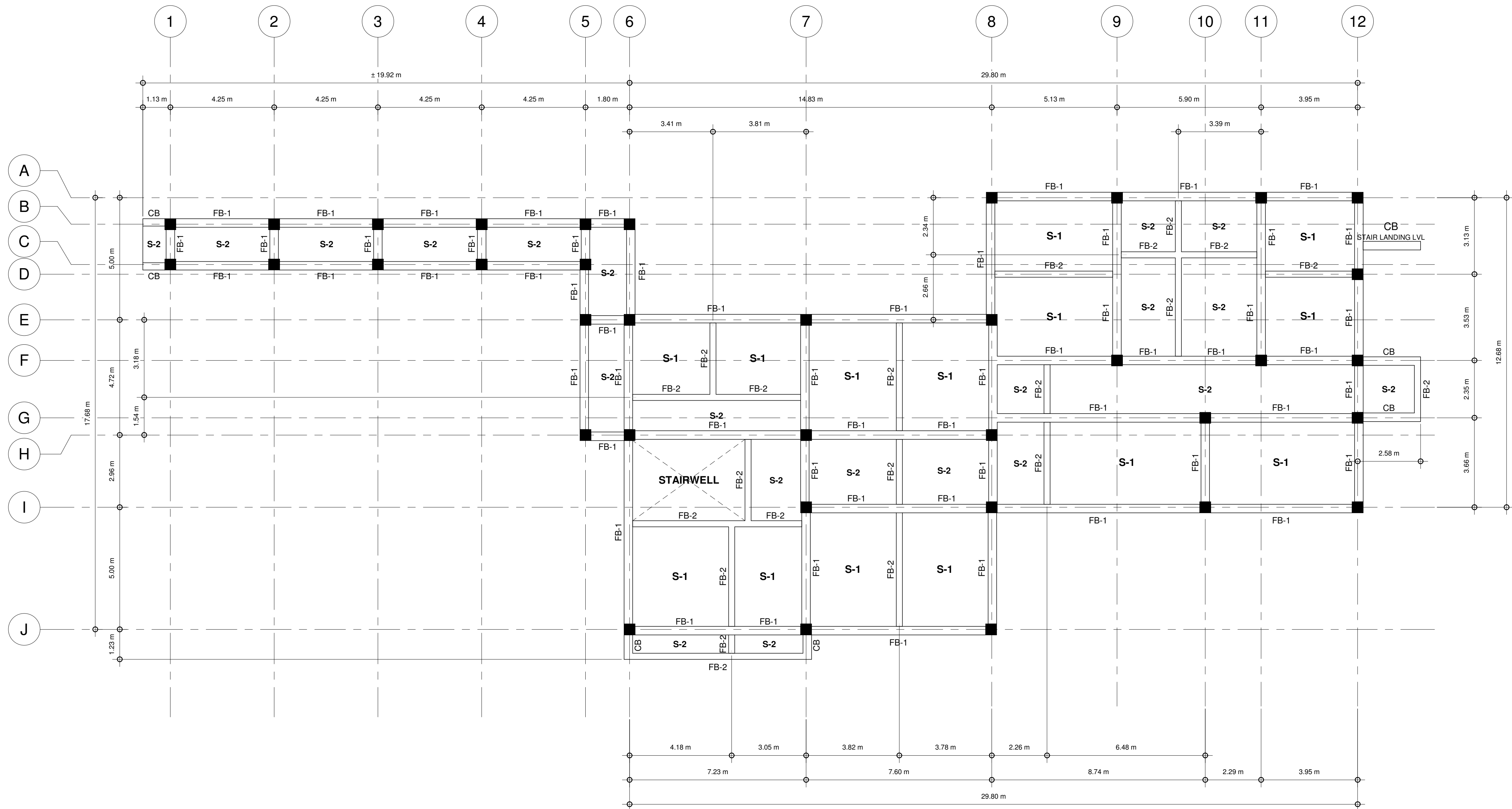
1 SECOND FLOOR FRAMING PLAN 1 : 100 meters
